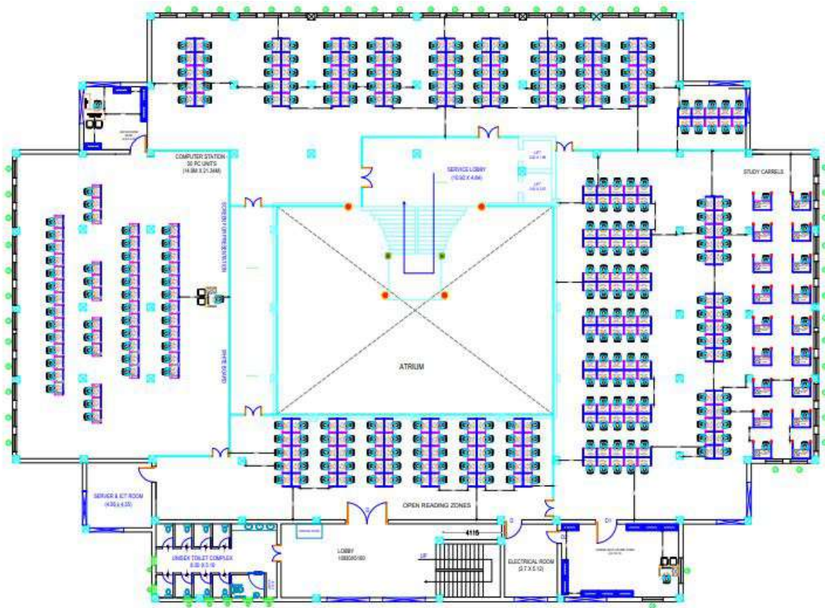
NLU LIBRARY BLOCK FIRST FLOOR
