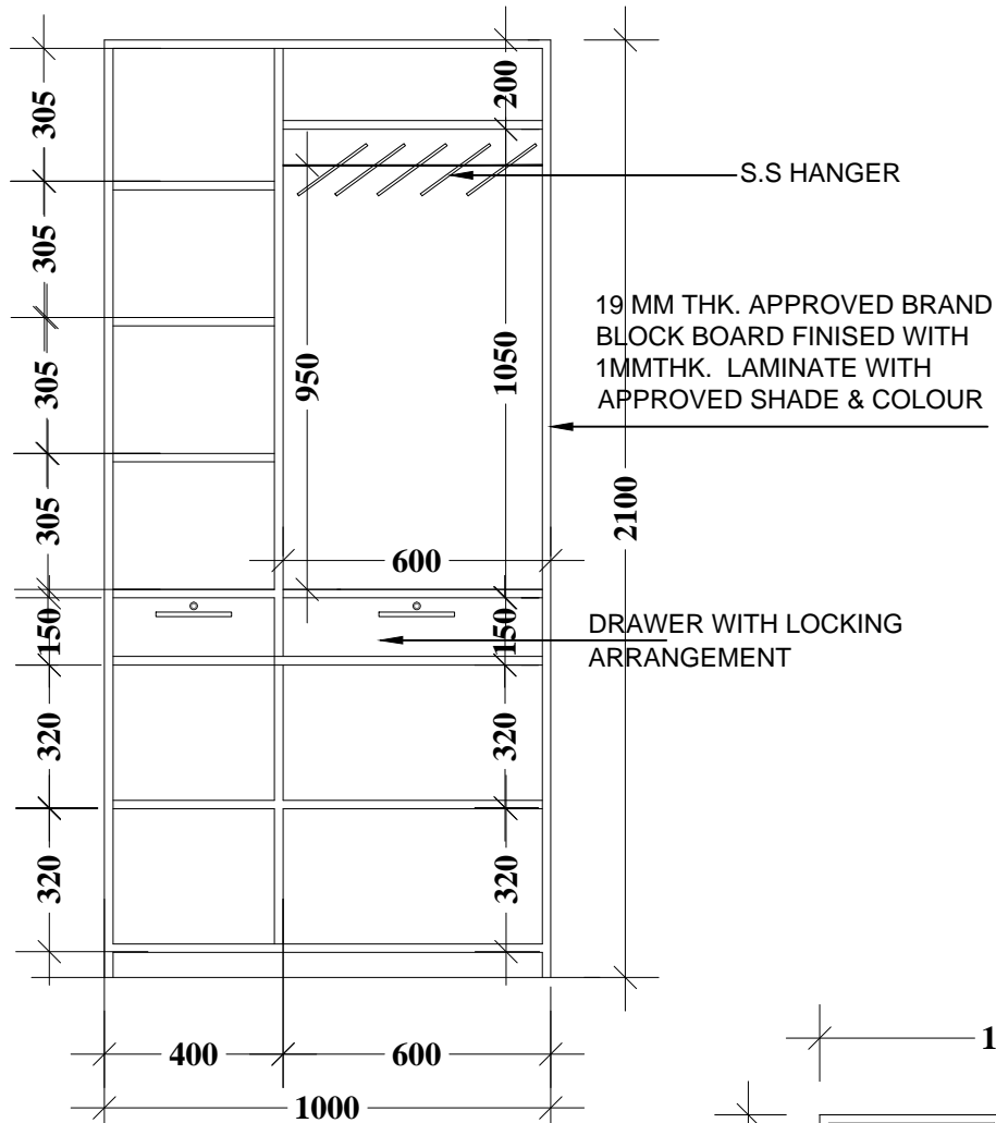
SECTION THROUGH X-X
