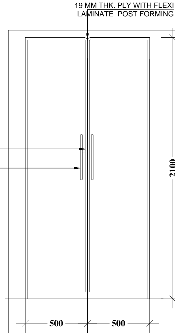
ELEVATION OF WARDROBE SIZE(1000X550X2100)
