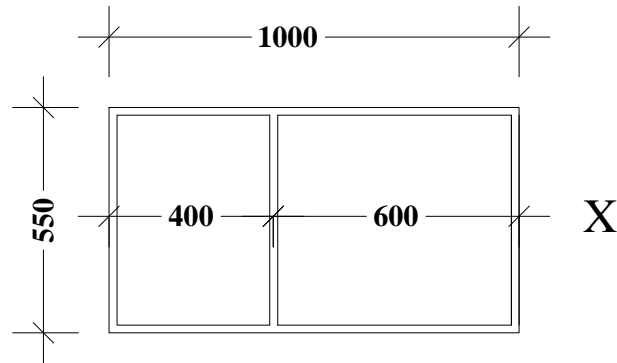
PLAN OF WARDROBE SIZE(1000X550X2100)
